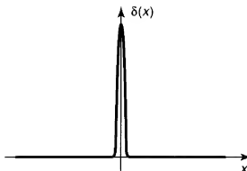
Figure 2.8: The Dirac delta function (Equation 2.93).
