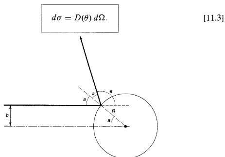
Figure 11.2: Elastic hard-sphere scattering.
