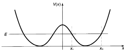
Figure 8.13: Symmetric double well; Problem 8.15.
