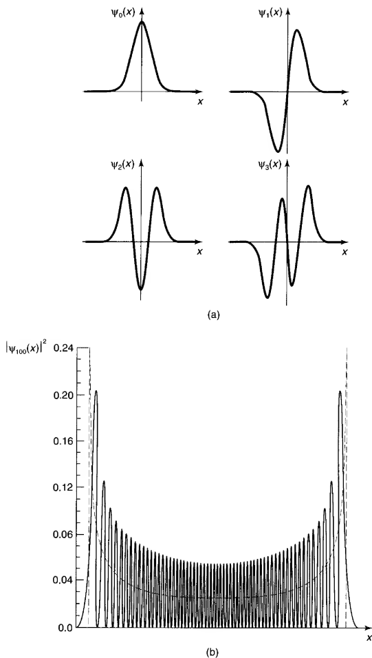
Figure 2.5: (a) The first four stationary states of the harmonic oscillator. (b) Graph of |\psi_{100}|^2 , with the classical distribution (dashed curve) superimposed.
