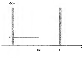
Figure 6.3: Constant perturbation over half the well.
