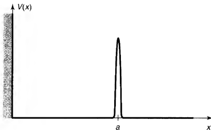
Figure 2.18: The potential for Problem 2.46.
