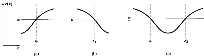
Figure 8.11: Upward-sloping and downward-sloping turning points.
