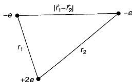
Figure 7.3: The helium atom.
