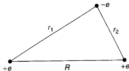
Figure 7.5: The hydrogen molecule ion, H_2^+ .
