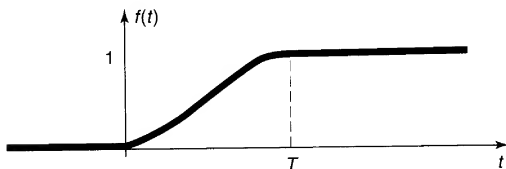
Figure 10.4: The function f(t) , in Equation 10.7.
