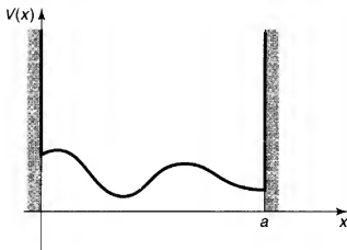
Figure 8.2: Infinite square well with a bumpy bottom.
