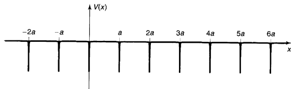
Figure 5.5: The Dirac comb, Equation 5.57.
