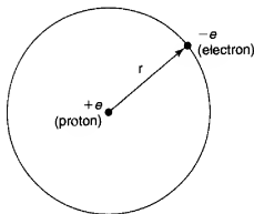
Figure 4.3: The hydrogen atom.
