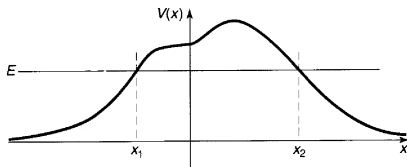
Figure 8.12: Barrier with sloping walls.
