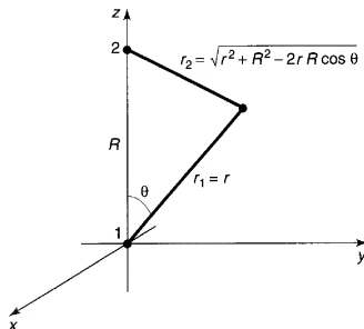
Figure 7.6: Coordinates for the calculation of I (Equation 7.39).
