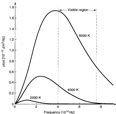
Figure 5.9: Planck's formula for the blackbody spectrum, Equation 5.112.
