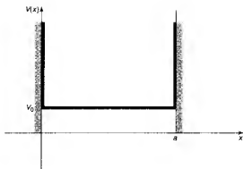
Figure 6.2: Constant perturbation over the whole well.
