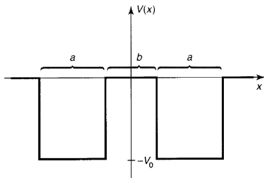
Figure 2.17: The double square well (Problem 2.44).
