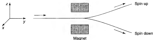
Figure 4.8: The Stern-Gerlach apparatus.
