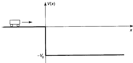
Figure 2.16: Scattering from a “cliff” (Problem 2.41).
