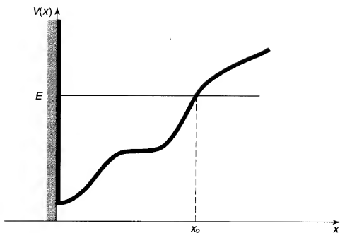
Figure 8.10: Potential well with one vertical wall.
