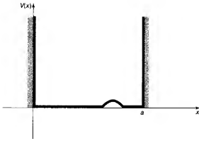
Figure 6.1: Infinite square well with small perturbation.
