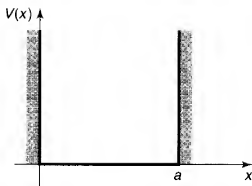
Figure 2.1: The infinite square well potential (Equation 2.15).
