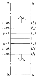
Figure 4.6: The “ladder” of angular momentum states.
