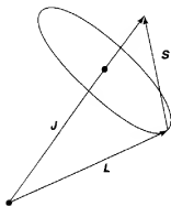
Figure 6.10: In the presence of spin-orbit coupling, \mathbf{L} and \mathbf{S} are not separately conserved; they precess about the fixed total angular momentum, \mathbf{J} .
