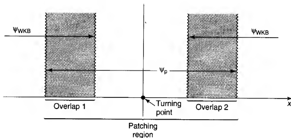
Figure 8.9: Patching region and the two overlap zones.
