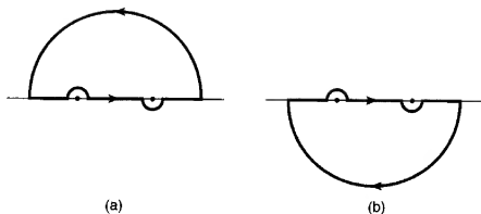
Figure 11.9: Closing the contour in equations [11.53] and [11.54].
