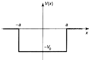
Figure 2.12: The finite square well (Equation 2.127).
