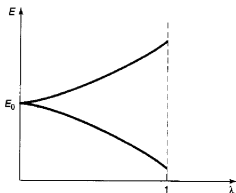
Figure 6.4: “Lifting” of a degeneracy by a perturbation.
