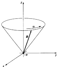
Figure 10.5: Magnetic field sweeps around on a cone, at angular velocity \omega , Equation 10.24.
