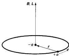
Figure 6.7: Hydrogen atom, from the electron's perspective.
