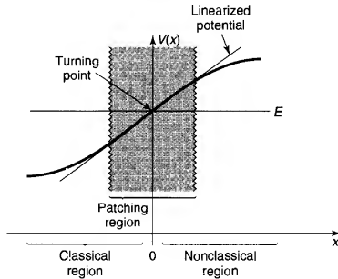
Figure 8.7: Enlarged view of the right-hand turning point.
