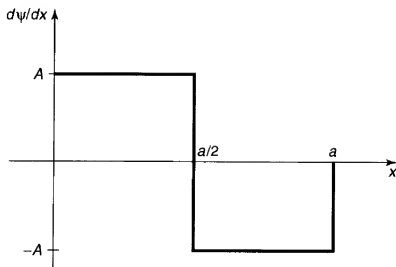
Figure 7.2: Derivative of the wave function in Figure 7.1.
