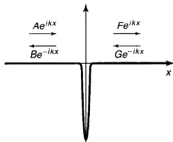
Figure 2.10: Scattering from a delta-function well.
