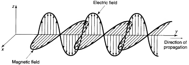
Figure 9.3: An electromagnetic wave.
