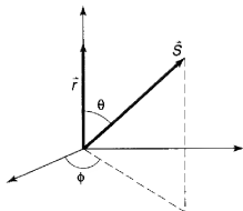
Figure 11.7: Convenient coordinates for the integral in equation [11.48].
